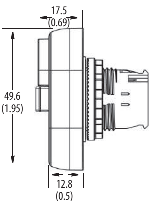
Non-illuminated 3-position Multi-function Operators
