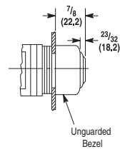
Square Backlit with Unguarded Bezel
