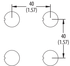
Emergency Stop
